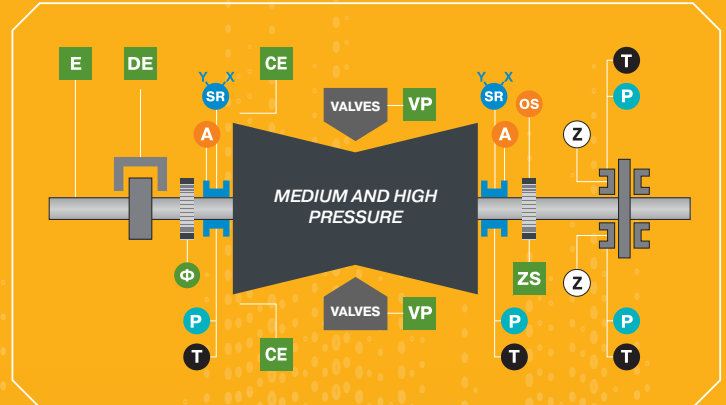
MEDIUM AND HIGH PRESSURE TURBINE
